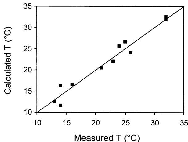
Fig. 3. Measured temperature vs. temperature calculated from mean Mg/Ca ratios for each month. Diagonal line is where T_{\text{measured}} = T_{\text{calculated}} .
