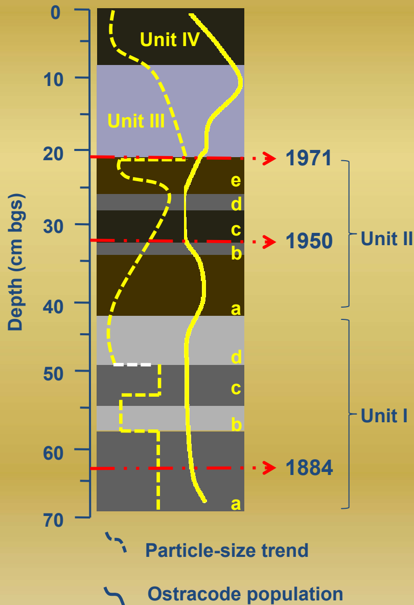
Figure 1. Ostracode biomass response to changes in sediment discharge due to damming of the stream.
