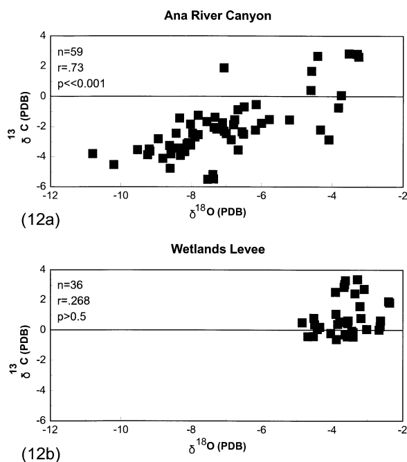
Figure 12. Cross plots of \delta^{18}\text{O} vs. \delta^{13}\text{C} for both Ana River Canyon (12a) and Wetlands Levee (12b) data.
