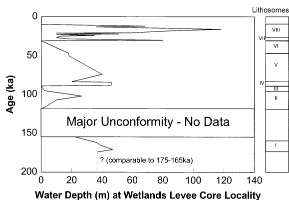
Figure 3. Lake Chewaucan lake level history for the past 200,000 yr. The curve shown is an estimate of water depth at the Wetlands Levee site, using lithologic and paleoecologic indicators at this locality and contemporaneous indicators at the other sites. This method of plotting lake level fluctuations was chosen over lake surface elevation because there has been significant sedimentary aggradation of the lake floor over the study interval, complicating comparisons of absolute lake surface elevations. Lake level estimation methods are discussed in the text. The Late Pleistocene (post 30,000 yr) record is based on a combination of data from this study and earlier work by Negrini & Davis (1992) and Negrini (submitted), and incorporates terrace elevation as well as core data.
