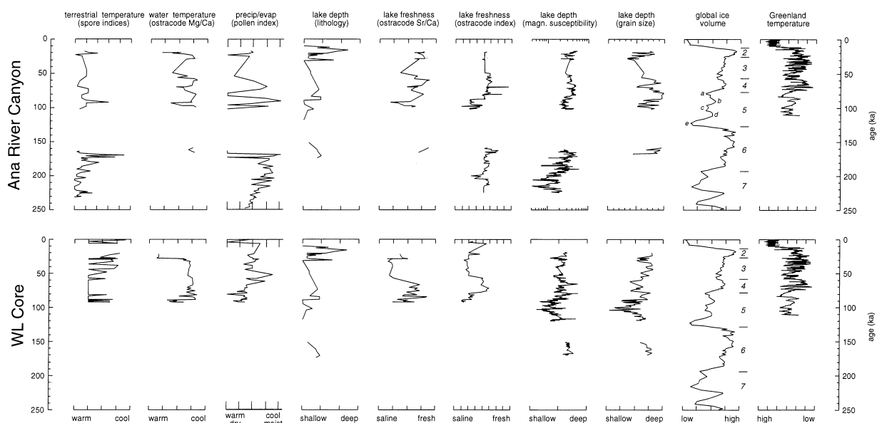
Figure 16. Key paleoenvironmental proxies from the Lake Chewaucan record, compared with the marine oxygen isotope record of Martinson et al. (1987) and the Greenland Ice Sheet isotopic record (Groote et al., 1993).
