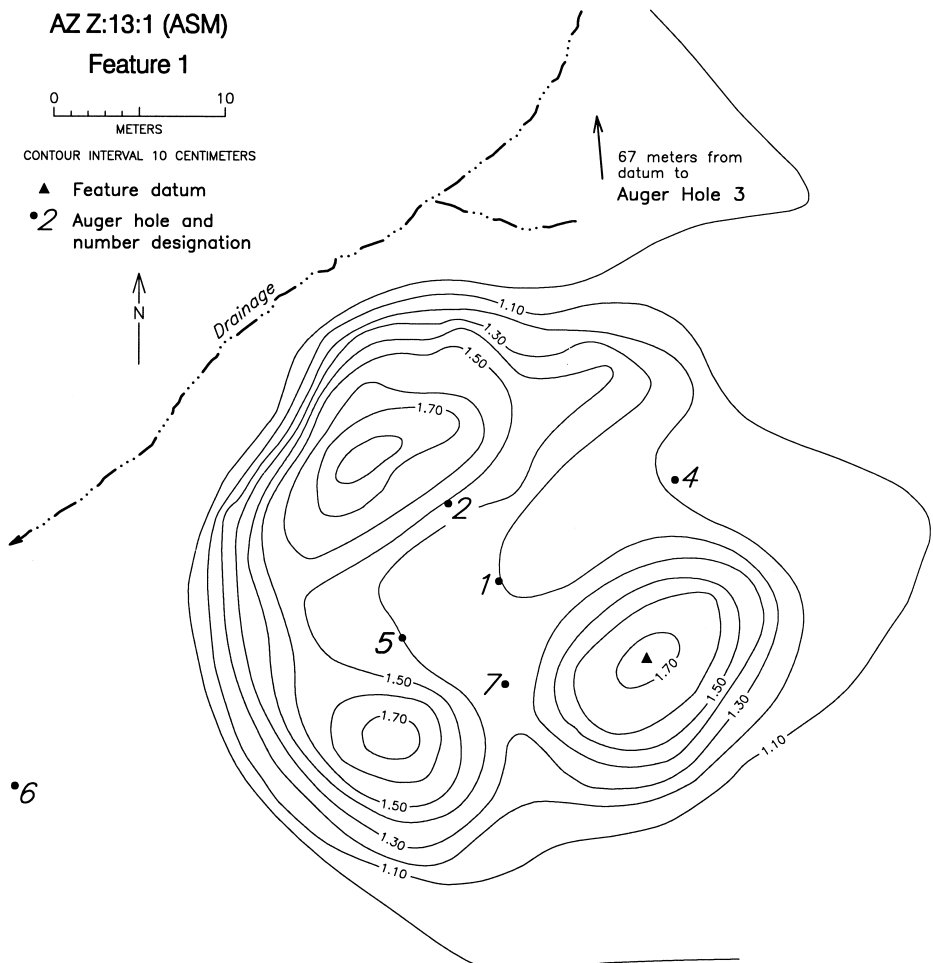
Figure 2. Contour map of the reservoir at archaeological site AZ Z:13:1 [ASM]. Note the locations of auger holes.
