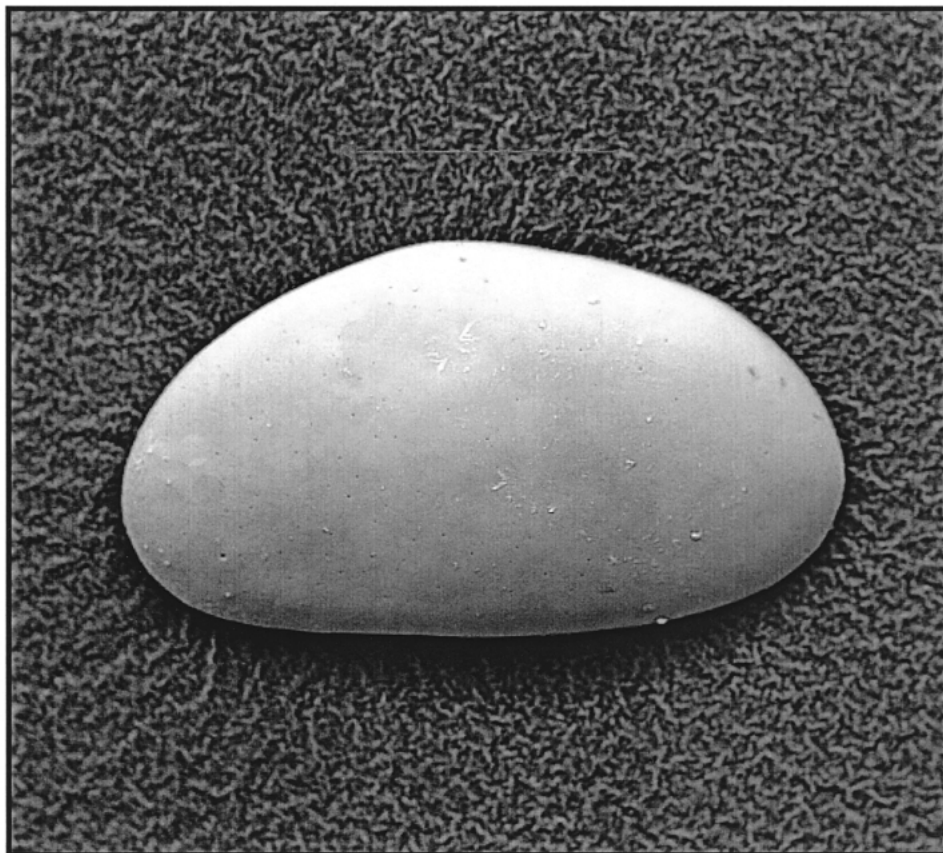
Figure 4. Scanning electron microscope (SEM) image of one of the Heterocypris antilliensis (Broodbakker, 1982) ostracodes recovered from the reservoir auger samples at site AZ Z:13:1 (ASM).
