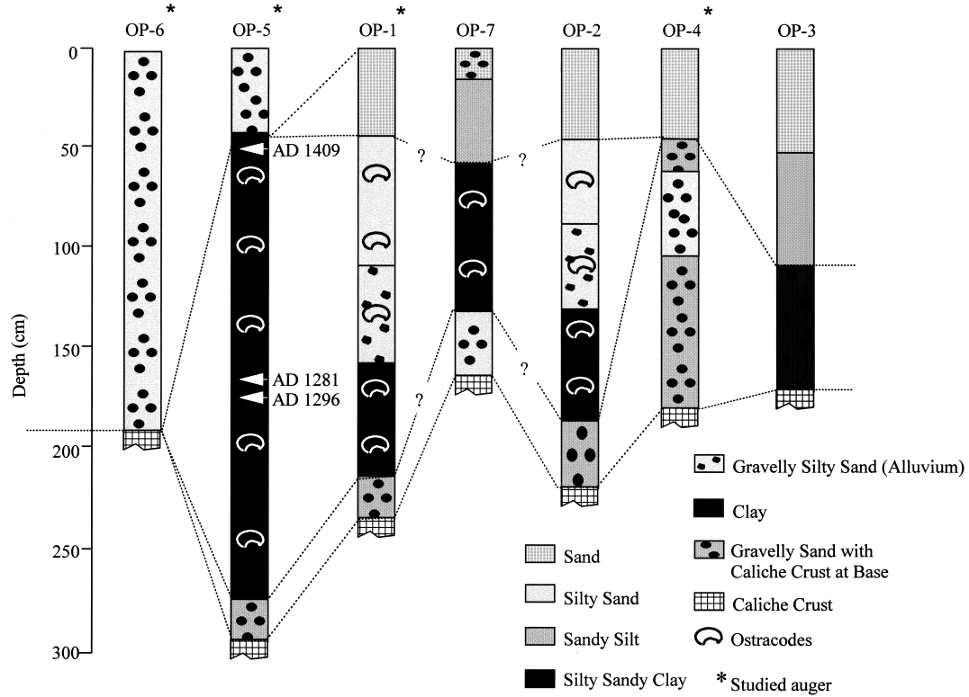
Figure 3. Stratigraphic profile of the auger columns in the reservoir. Note the vertical locations of ostracodes. The profile of OP-5 shows the location of radiocarbon age-estimations.
